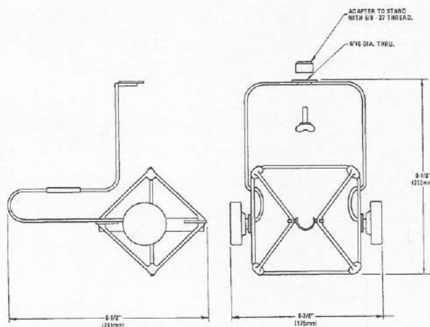
FIGURE 1—Dimensions
