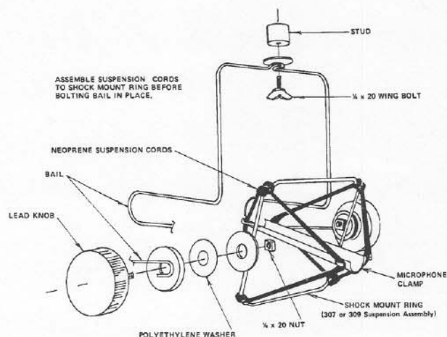
FIGURE 2—Assembly Drawing
